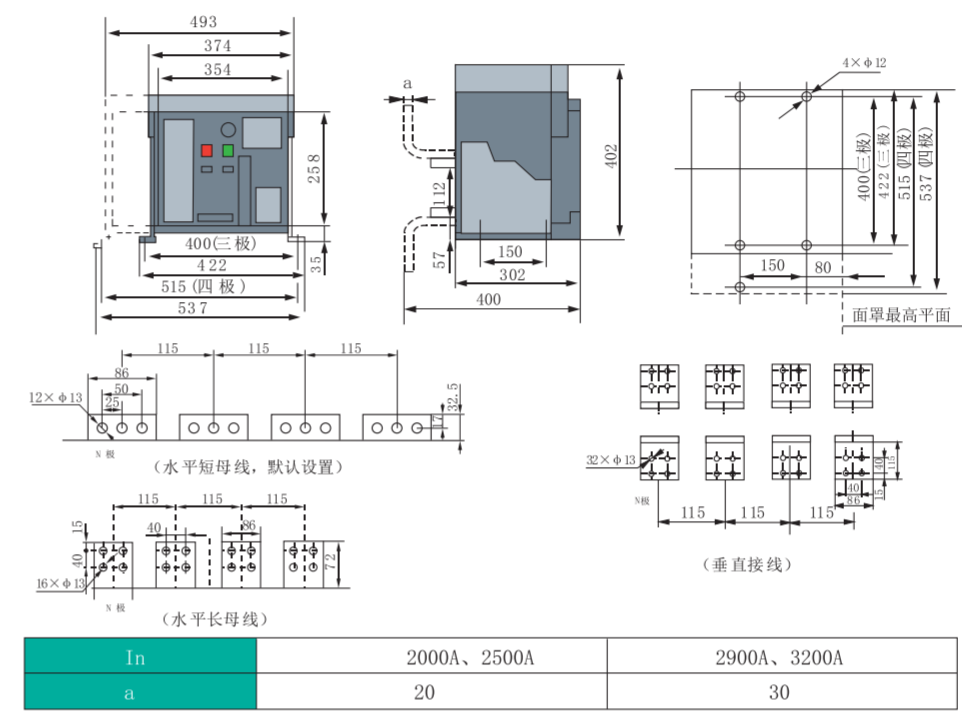
19.6 TGW1N-3200/TGW1N-3200H 抽屉式断路器外形尺寸与安装尺寸图
