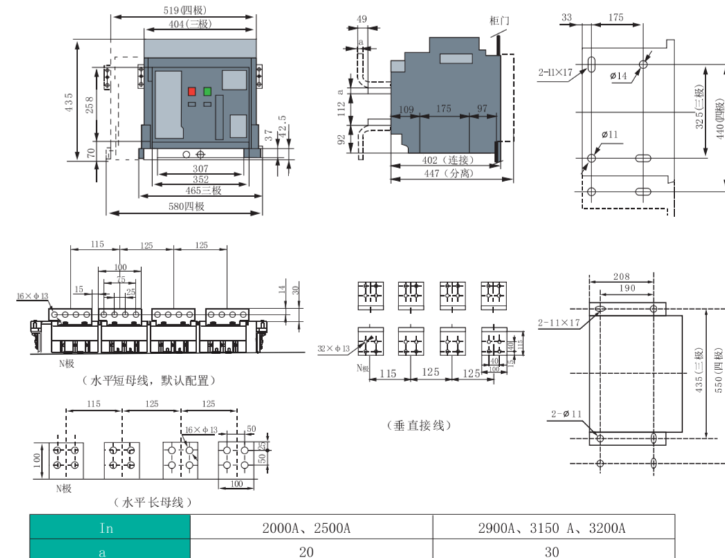
19.6 TGW1N-3200/TGW1N-3200H 抽屉式断路器外形尺寸与安装尺寸图
